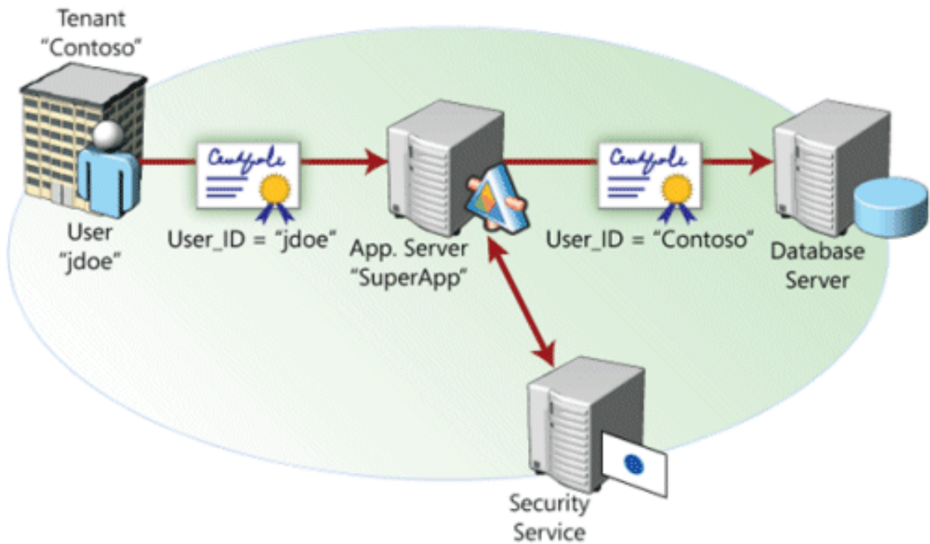
Figure 8. A SaaS application connects to a database using a combination of the impersonation and trusted subsystem approaches
