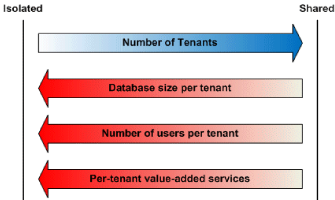
Figure 5. Tenant-related factors and how they affect “isolated versus shared” data architecture decisions
